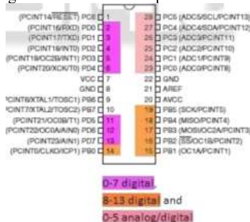
Fig. 5: Pin Diagram of Atmega328P
